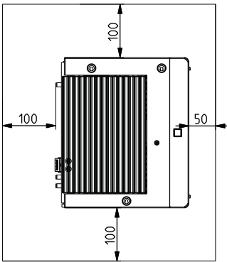
Fig. 1: Clearances to containing surfaces
