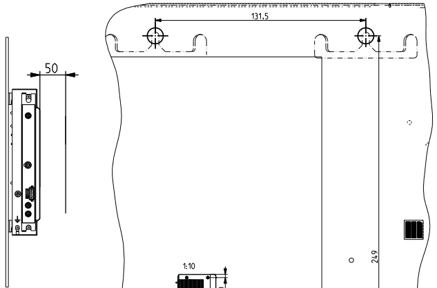
Fig. 2: Dimensions and installation dimensions
